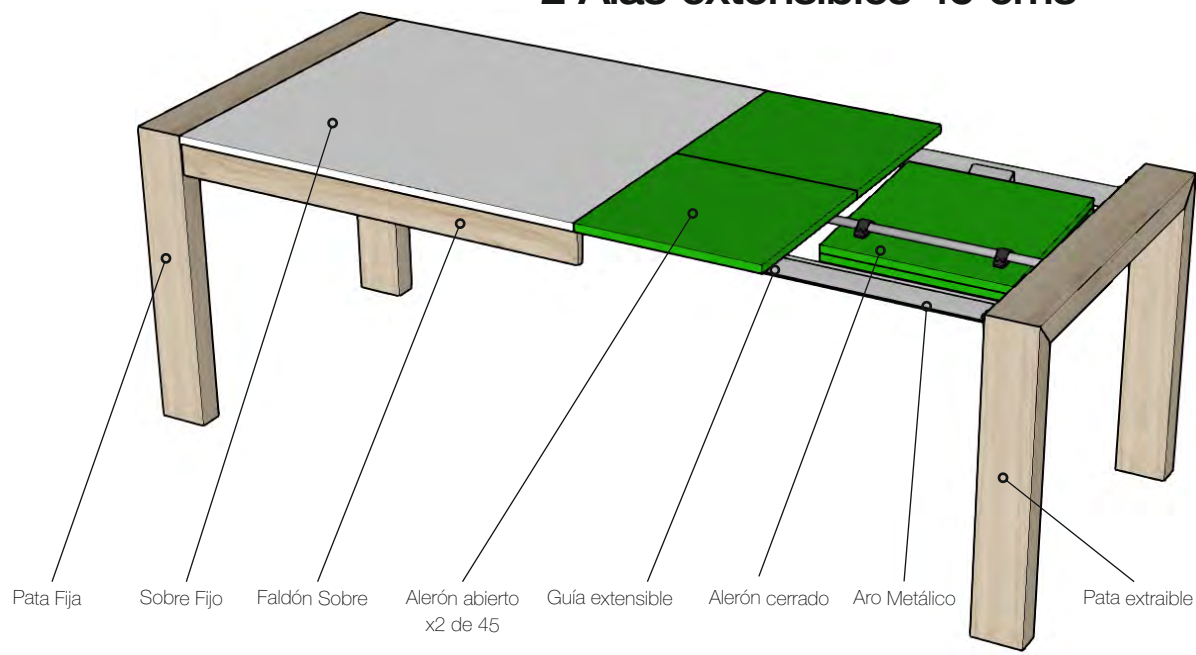
Mesa Mod. “U” 2 Alas extensibles 45 cms
